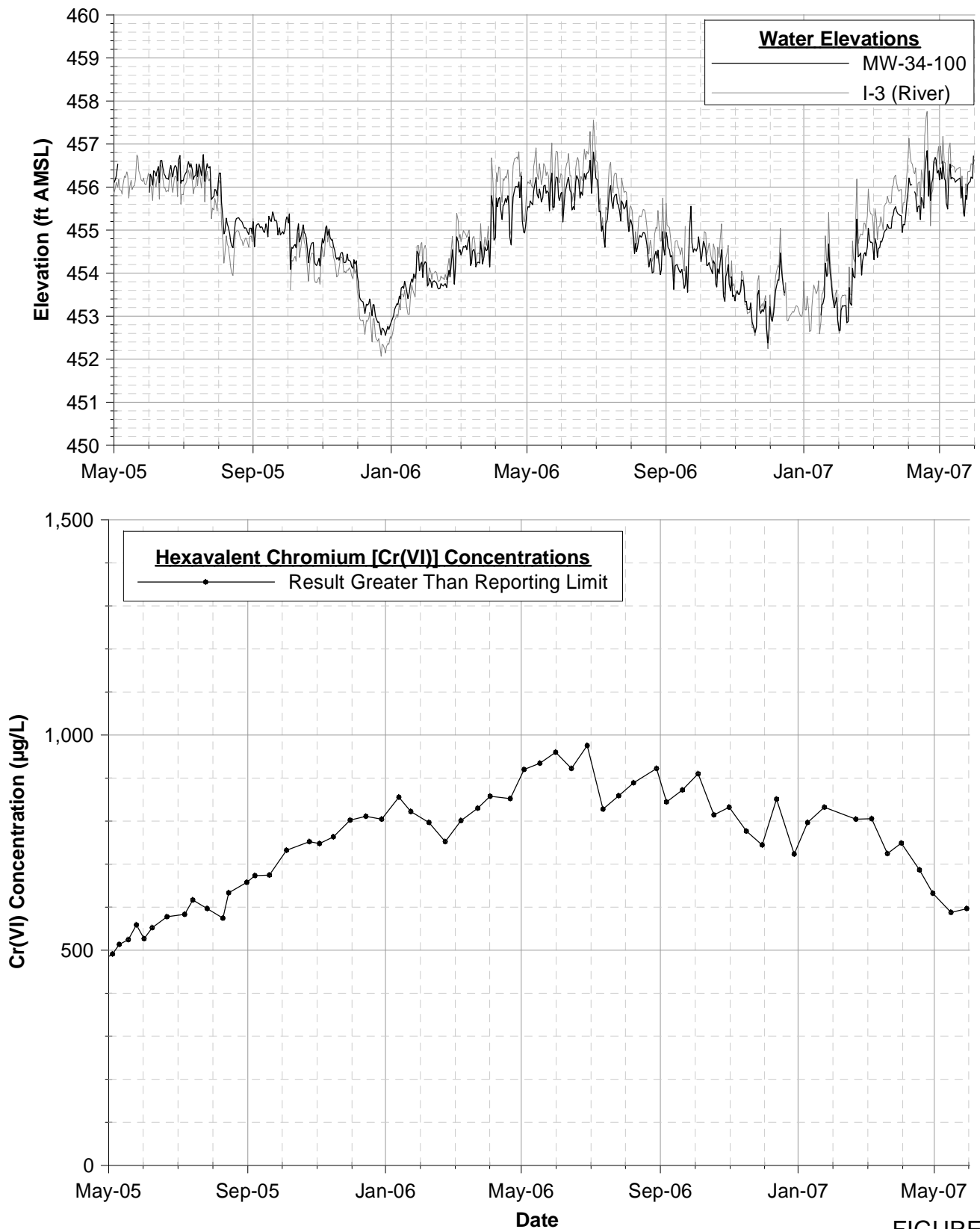
FIGURE B-2 MW-34-100 CR(VI) CONCENTRATION & HYDROGRAPH - 5/1/2005 - 5/30/2007 INTERIM MEASURES PERFORMANCE MONITORING PG&E TOPOCK COMPRESSOR STATION NEEDLES, CALIFORNIA
