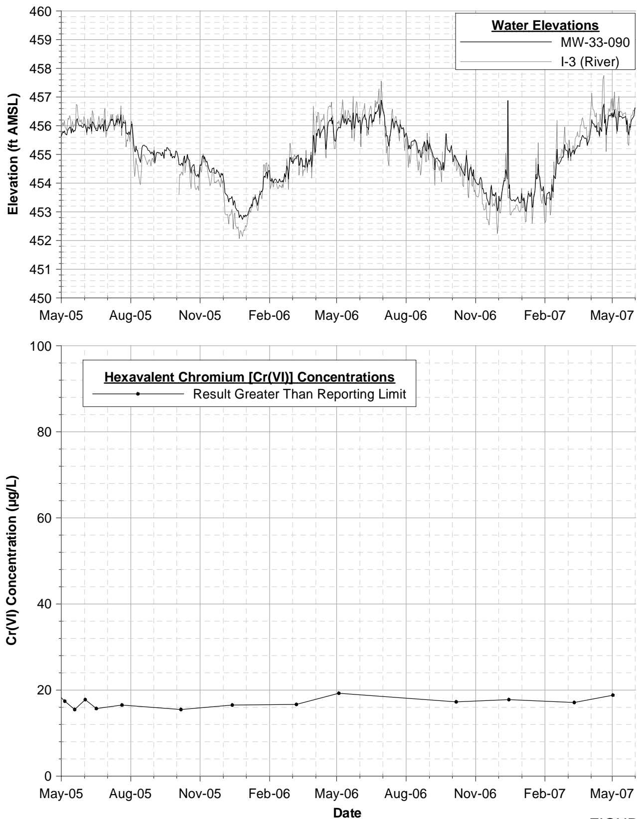
FIGURE B-1 MW-33-90 CR(VI) CONCENTRATION & HYDROGRAPH - 5/1/2005 - 5/2/2007 INTERIM MEASURES PERFORMANCE MONITORING PG&E TOPOCK COMPRESSOR STATION NEEDLES, CALIFORNIA
