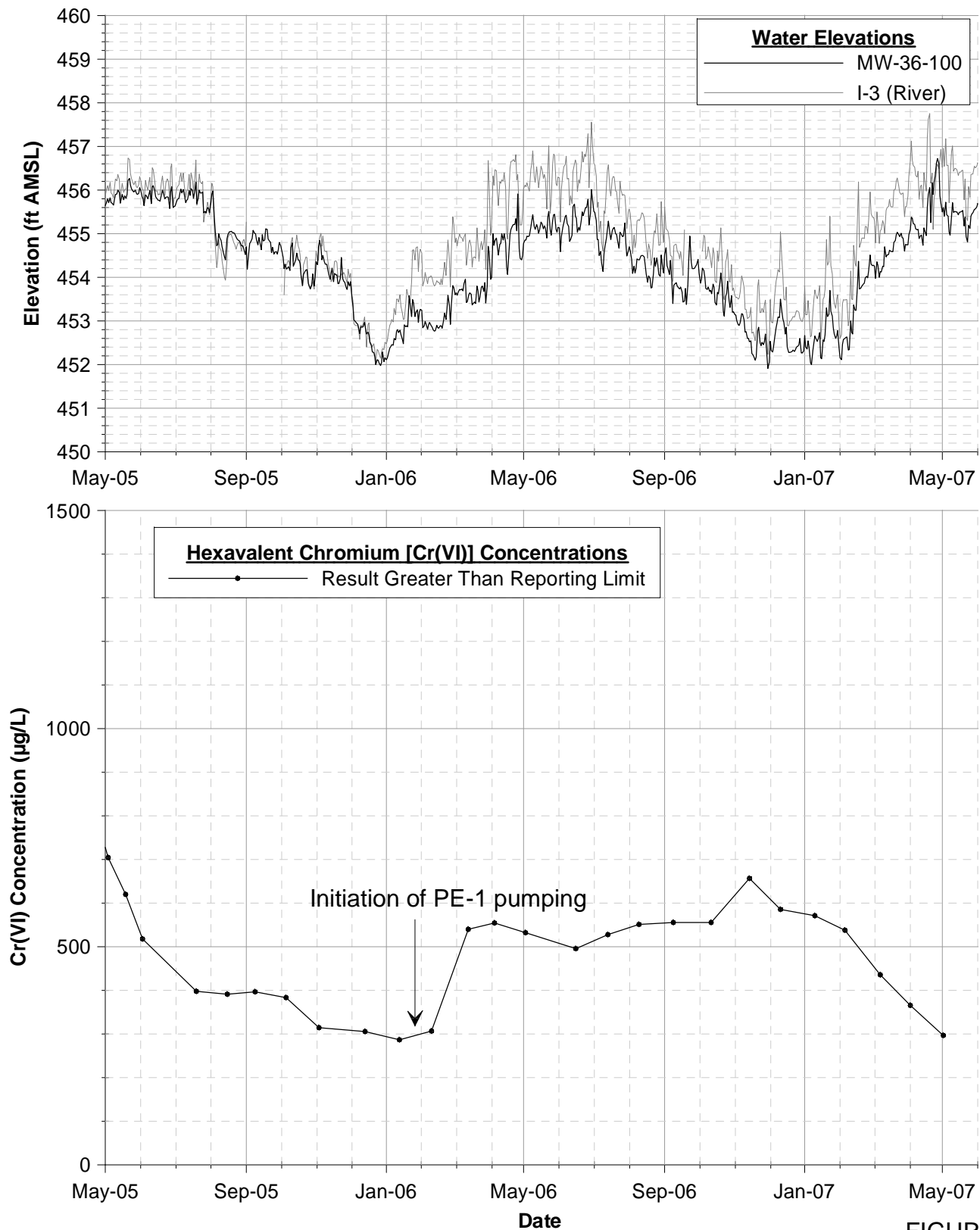
FIGURE B-3 MW-36-100 CR(VI) CONCENTRATION & HYDROGRAPH - 5/1/2005 - 5/2/2007 INTERIM MEASURES PERFORMANCE MONITORING PG&E TOPOCK COMPRESSOR STATION NEEDLES, CALIFORNIA
