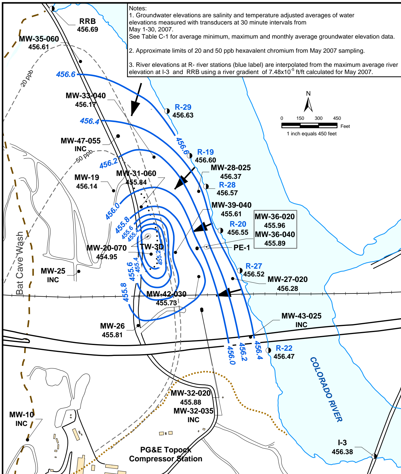
FIGURE 4-1 AVERAGE GROUNDWATER ELEVATIONS SHALLOW WELLS AND RIVER ELEVATIONS, MAY 2007
