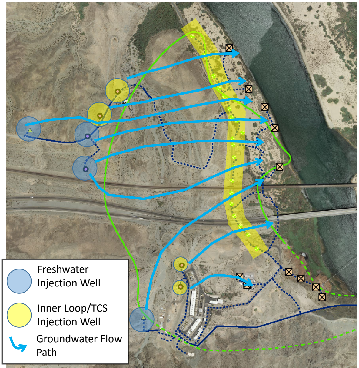
Groundwater Remedy Components: Injection Wells
